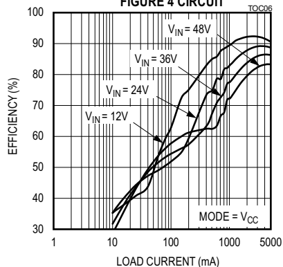
EFFICIENCY vs. LOAD CURRENT 3.3V OUTPUT, DCM MODE, FIGURE 4 CIRCUIT
