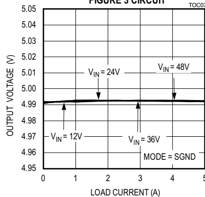
LOAD AND LINE REGULATION 5V OUTPUT, PWM MODE, FIGURE 3 CIRCUIT
