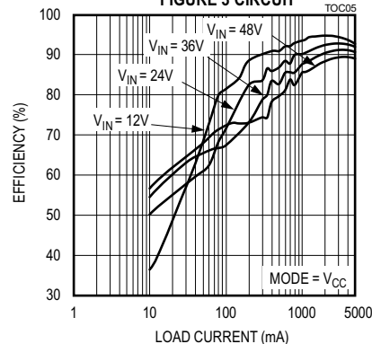
EFFICIENCY vs. LOAD CURRENT 5V OUTPUT, DCM MODE, FIGURE 3 CIRCUIT
