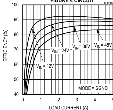
EFFICIENCY vs. LOAD CURRENT 3.3V OUTPUT, PWM MODE, FIGURE 4 CIRCUIT
