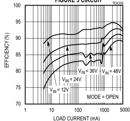
EFFICIENCY vs. LOAD CURRENT 5V OUTPUT, PFM MODE, FIGURE 3 CIRCUIT
