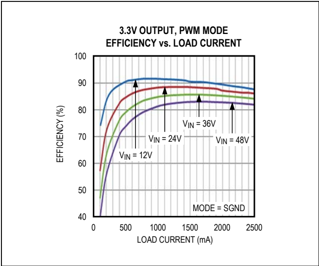
Figure 2. MAX17503 3.3V Output Efficiency (PWM Mode)
