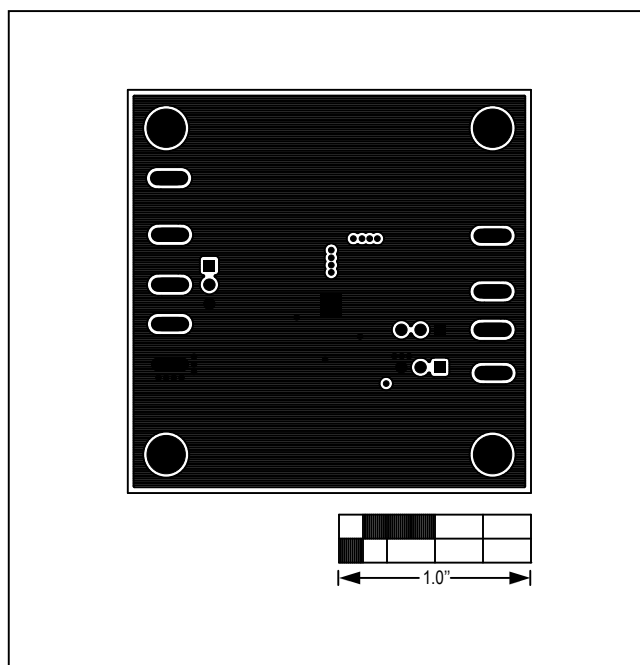
Figure 15. MAX17503 3.3V Output EV Kit PCB Layout—Inner Layer 2
