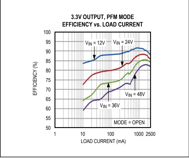
Figure 4. MAX17503 3.3V Output Efficiency (PFM Mode)
