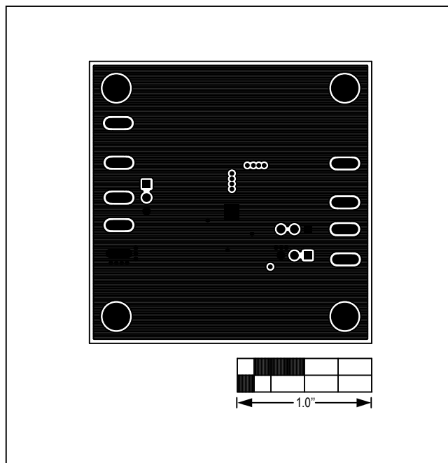
Figure 14. MAX17503 3.3V Output EV Kit PCB Layout—Inner Layer 1
