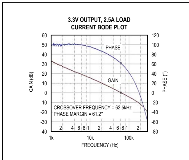
Figure 6. MAX17503 3.3V Output Full Load Bode Plot ( V_{IN} = 24V )
