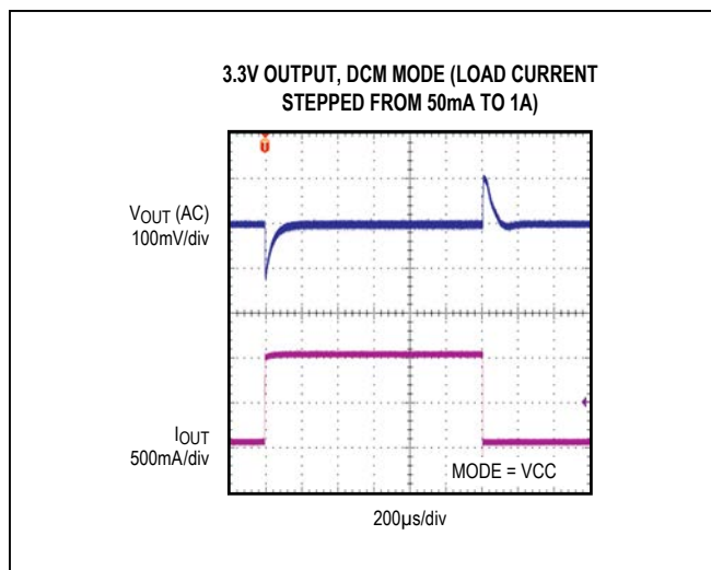
Figure 9. MAX17503 3.3V Output, 50mA to 1A Load Transient (DCM Mode)
