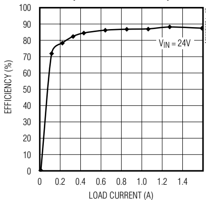
EFFICIENCY GRAPH AT 24V INPUT (FLYBACK REGULATOR)
