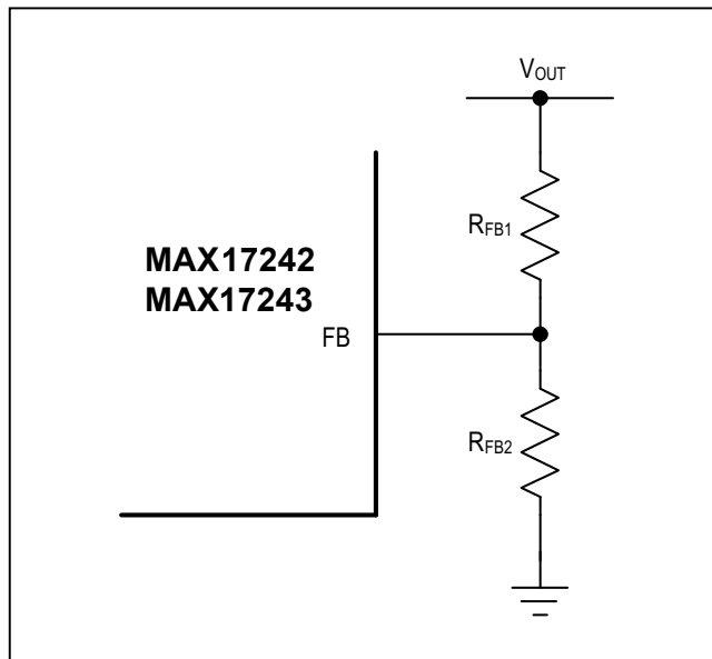
Figure 2. Adjustable Output-Voltage Setting
