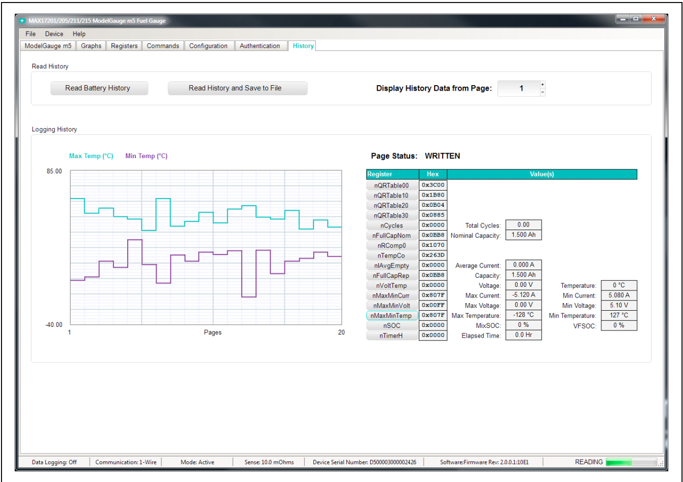
Figure 11. History Tab
