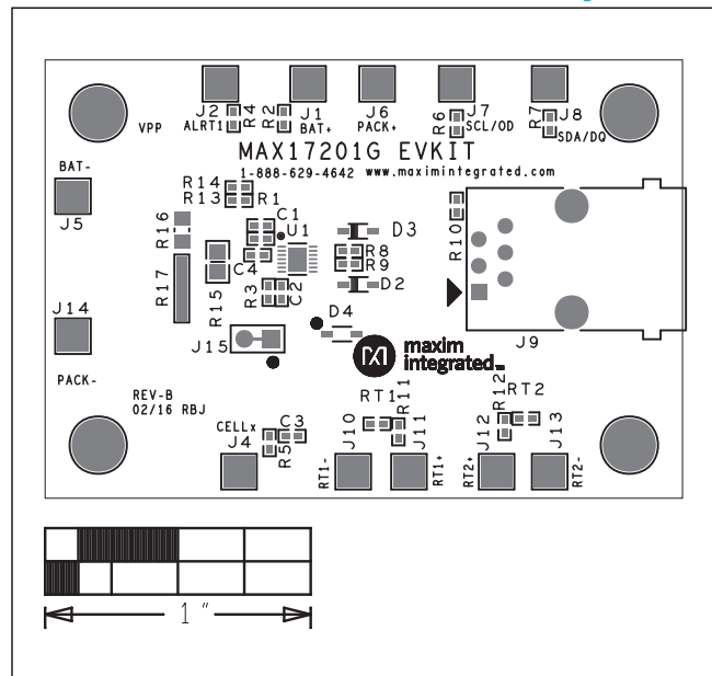
Component Placement
