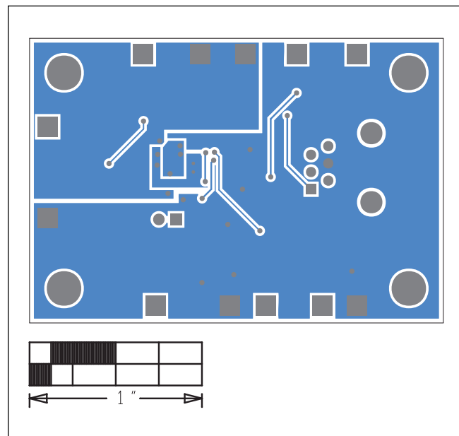
Bottom Layout
