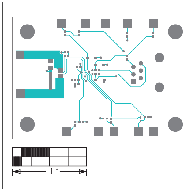
Top Layout
