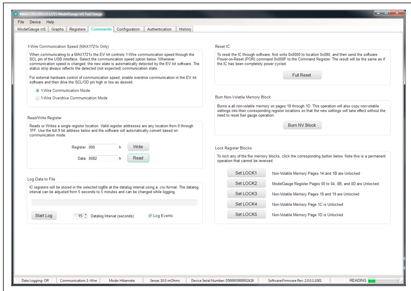
Figure 8. Commands Tab
