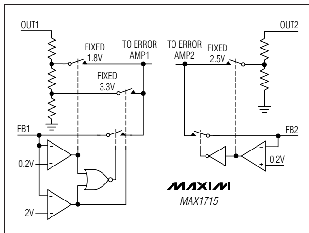
Figure 9. Feedback Mux
