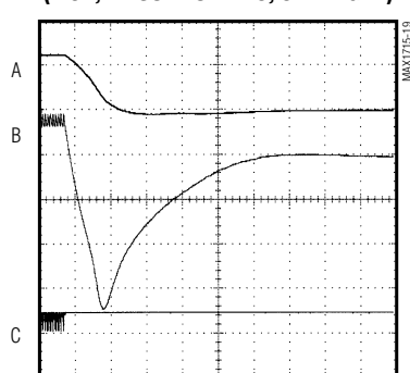
SHUTDOWN WAVEFORM (2.5V, 4A COMPONENTS, SKIP = GND)
