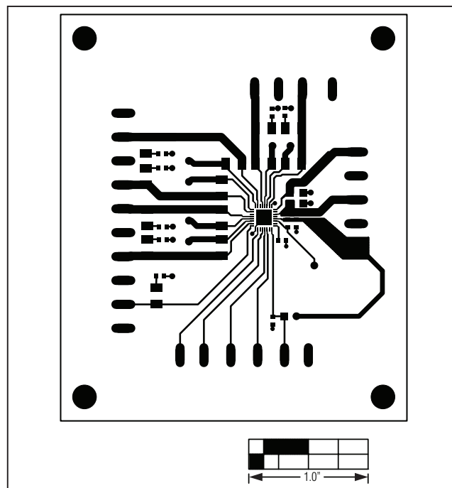
Figure 3. MAX17120 EV Kit PCB Layout—Component Side
