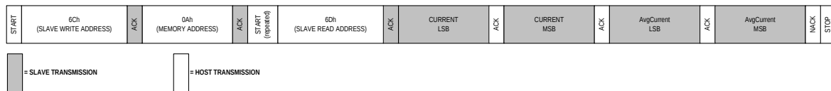
Figure 17. Example I 2 C read data communication sequence.
