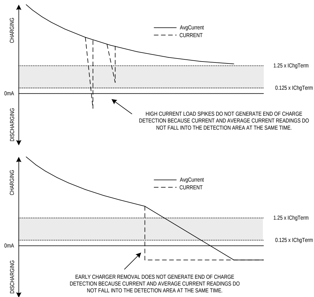
Figure 7. ModelGauge m5 rejects false end-of-charge events.
