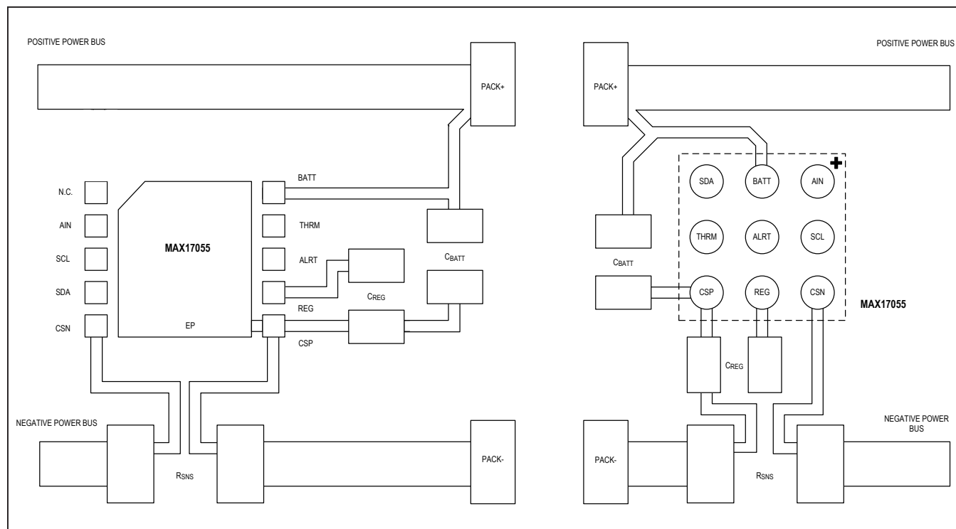
Figure 4. Layout Examples
