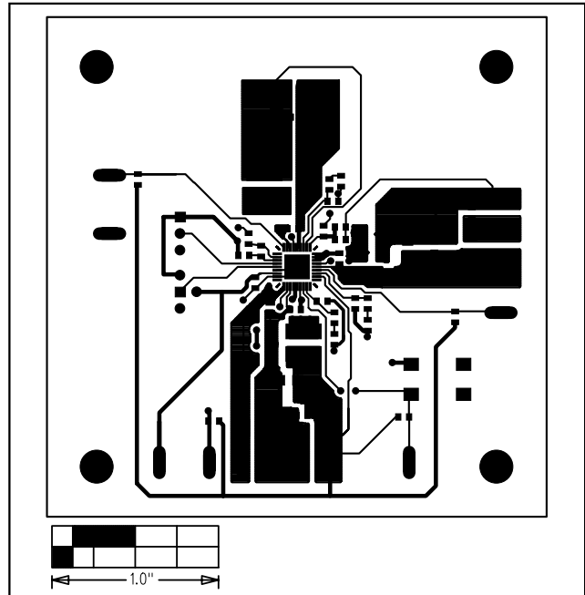
Figure 3. MAX1702 EV Kit PC Board Layout—Component Side
