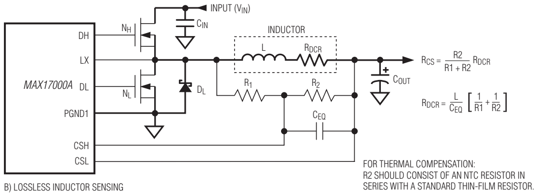
Figure 7b. Current-Sense Configurations (Sheet 2 of 2)
