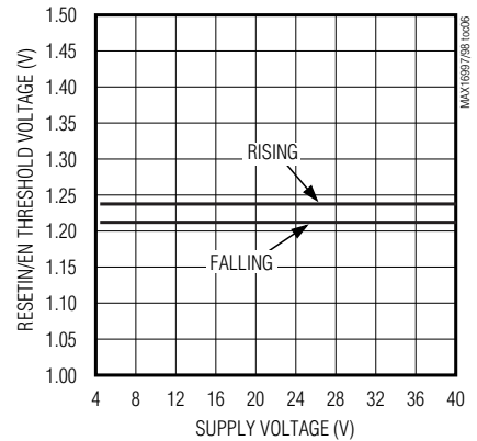
RESET/EN THRESHOLD VOLTAGE vs. SUPPLY VOLTAGE
