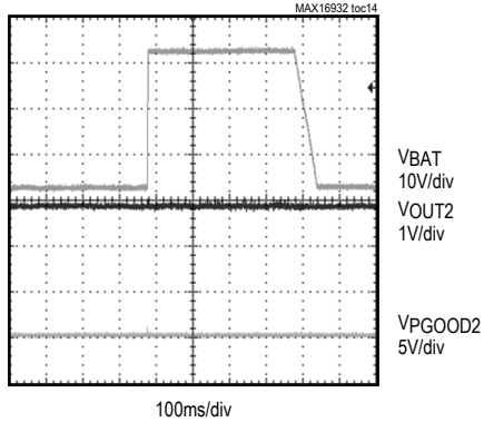
LOAD DUMP
