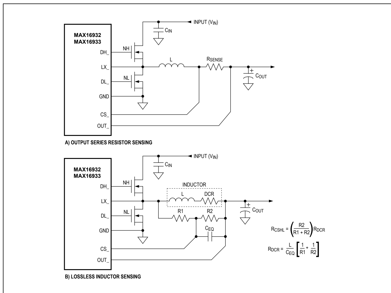
Figure 1. Current-Sense Configurations
