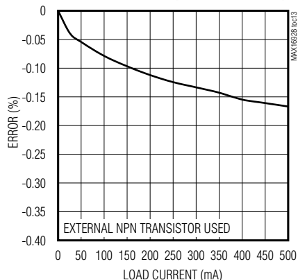
LOAD REGULATION (3.3V REGULATOR)
