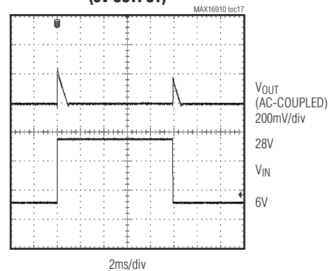
LINE-TRANSIENT RESPONSE (5V OUTPUT)
