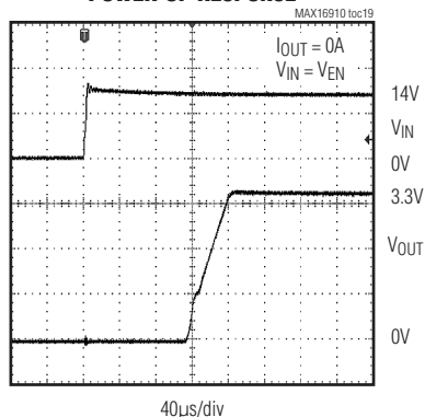
POWER-UP RESPONSE
