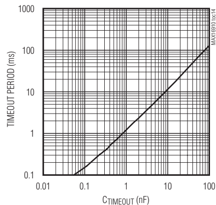
RESET TIMEOUT PERIOD vs. TIMEOUT CAPACITANCE
