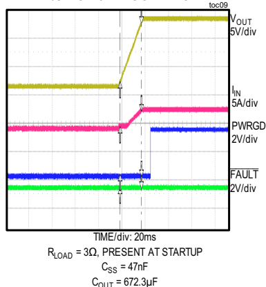
STARTUP INTO LOAD CONTROLLED WITH EN/UVLO—3Ω RESISTIVE LOAD
