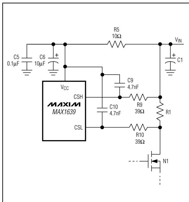
Figure 5. High-Side Current Sense
