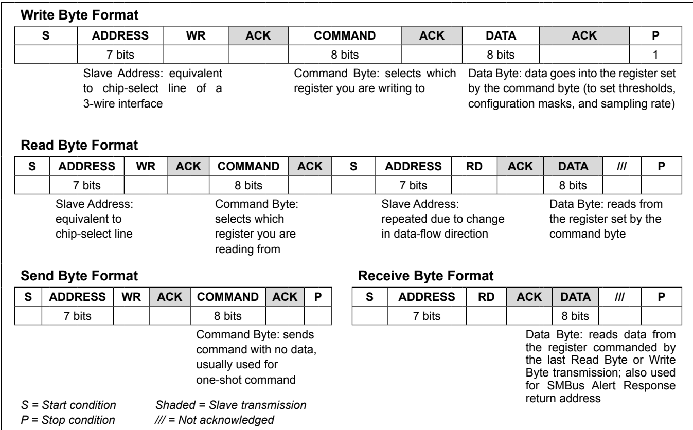
Figure 3. SMBus Protocols
