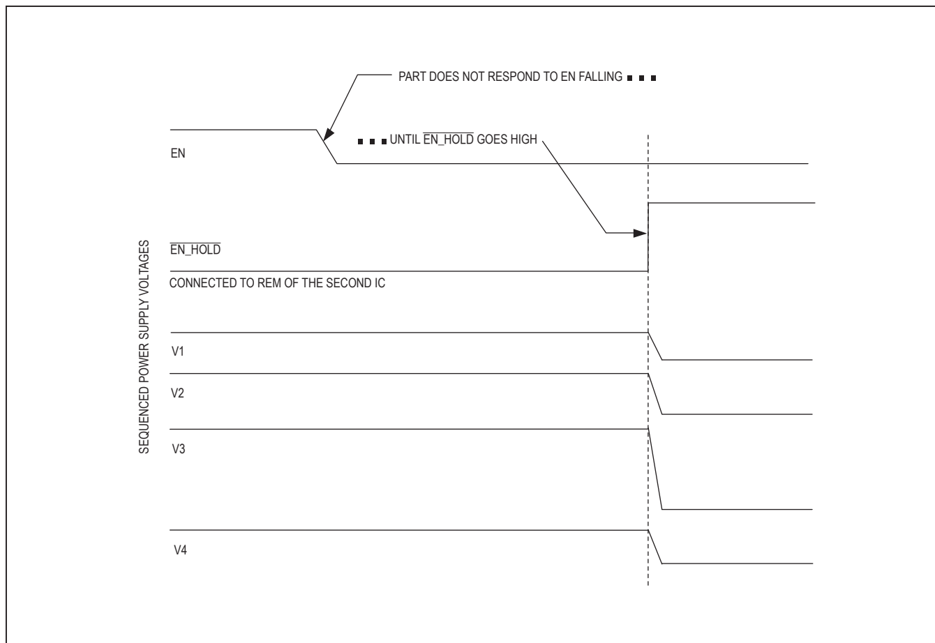
Figure 5. Power-Down Characteristics when REM of the Second IC is Connected to \overline{\text{EN\_HOLD}} of the First IC. See the Typical Application Circuit (Figure 1).
