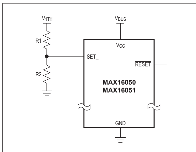
Figure 6. Setting the \text{SET\_} Input
