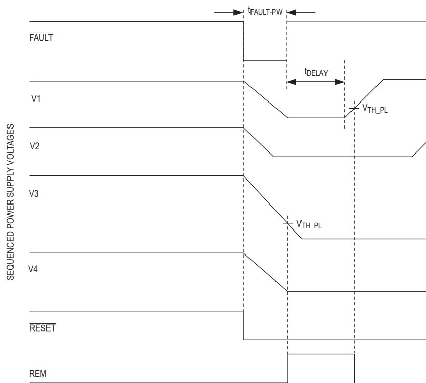
Figure 4. Sequencing Timing Diagram During a System Fault. See the Typical Application Circuit ( Figure 1 ).
