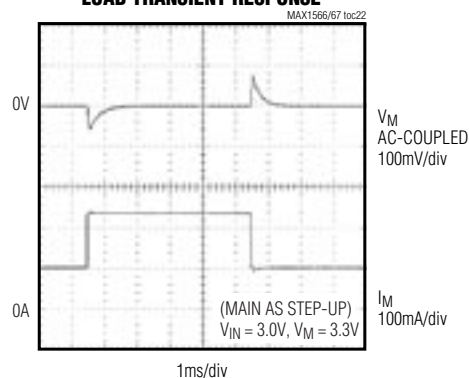
MAIN (STEP-UP MODE) LOAD TRANSIENT RESPONSE
