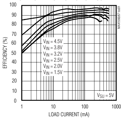
STEP-UP EFFICIENCY vs. LOAD CURRENT
