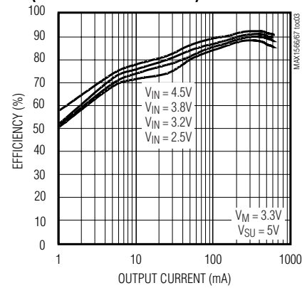
BOOST-BUCK EFFICIENCY (SU + MAIN AS STEP-DOWN) vs. LOAD CURRENT
