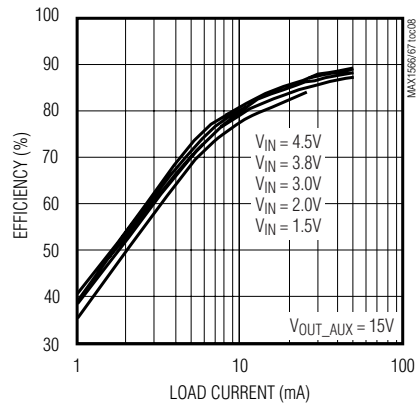
AUX EFFICIENCY vs. LOAD CURRENT
