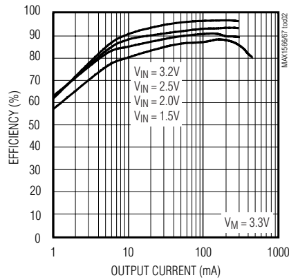
MAIN (STEP-UP) EFFICIENCY vs. LOAD CURRENT
