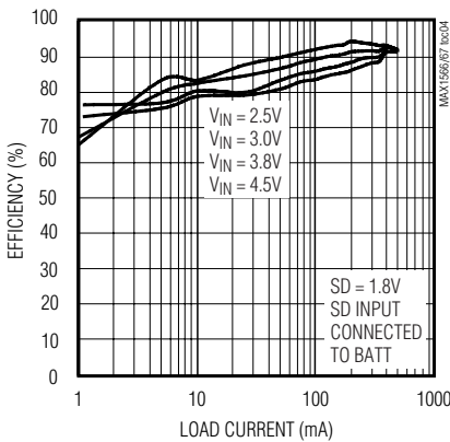
STEP-DOWN EFFICIENCY vs. LOAD CURRENT
