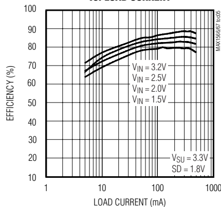
BOOST-BUCK EFFICIENCY (SU + SD) vs. LOAD CURRENT
