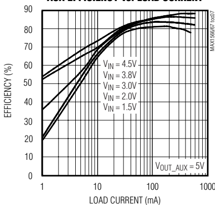
AUX EFFICIENCY vs. LOAD CURRENT
