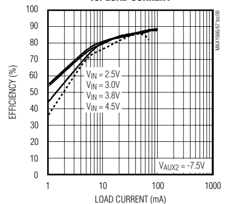
MAX1567 AUX2 EFFICIENCY vs. LOAD CURRENT
