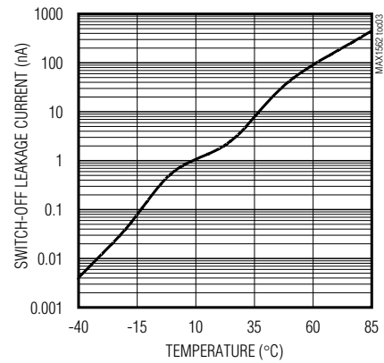
SWITCH-OFF LEAKAGE CURRENT vs. TEMPERATURE
