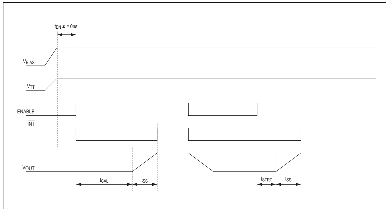
Figure 7. Startup Sequence
