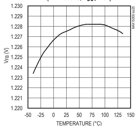
FB VOLTAGE vs. TEMPERATURE (MAX15007C, V OUT = 5V)
