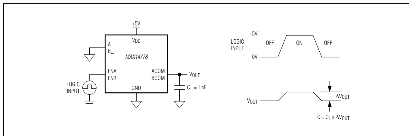
Figure 5. Charge Injection
