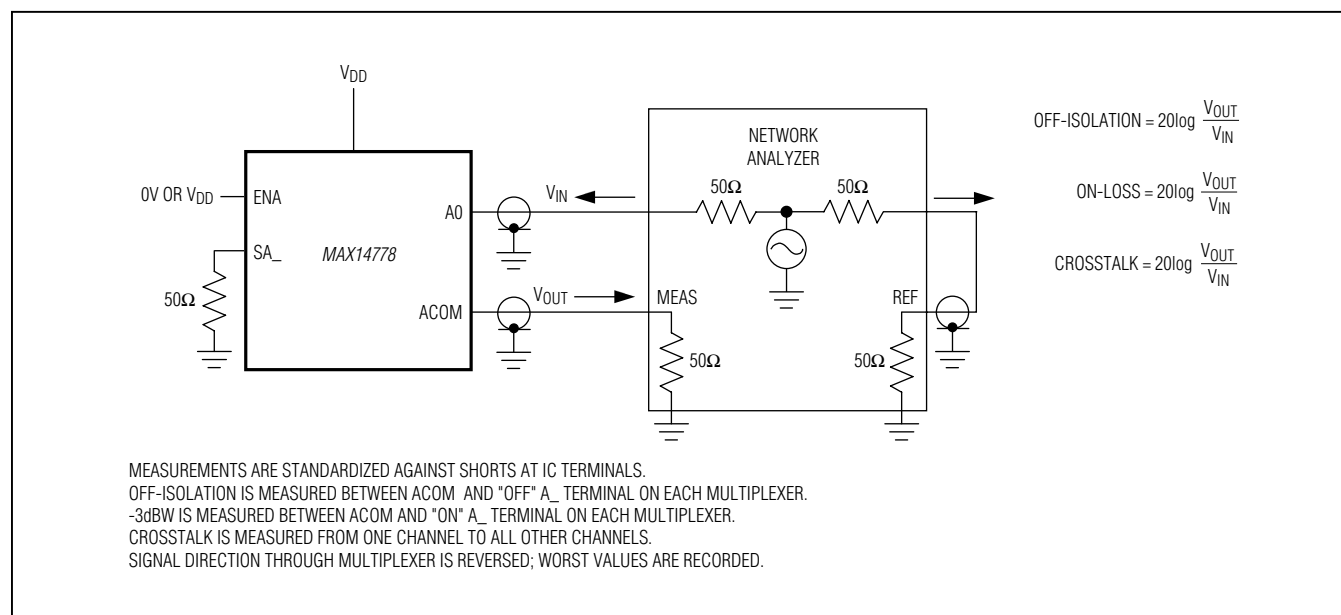
Figure 6. Off-Isolation, -3dB Bandwidth, and Crosstalk
