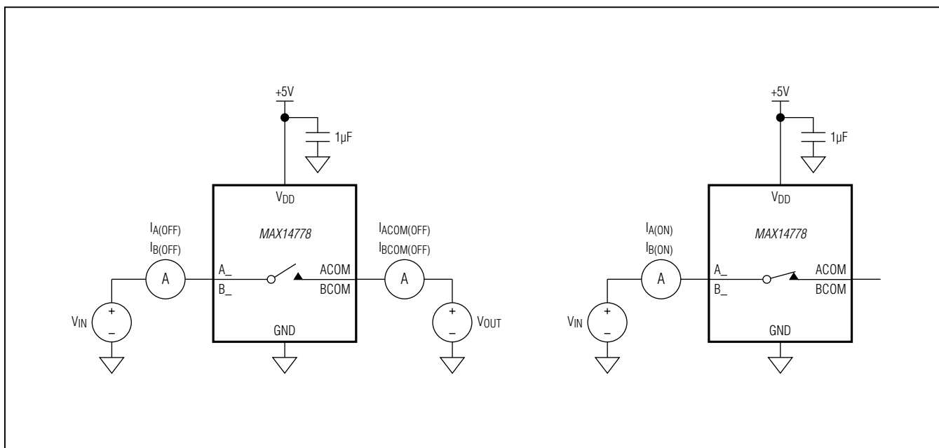
Figure 2. Leakage Current Measurement
