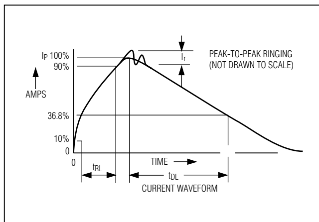
Figure 11. Human Body Current Waveform
