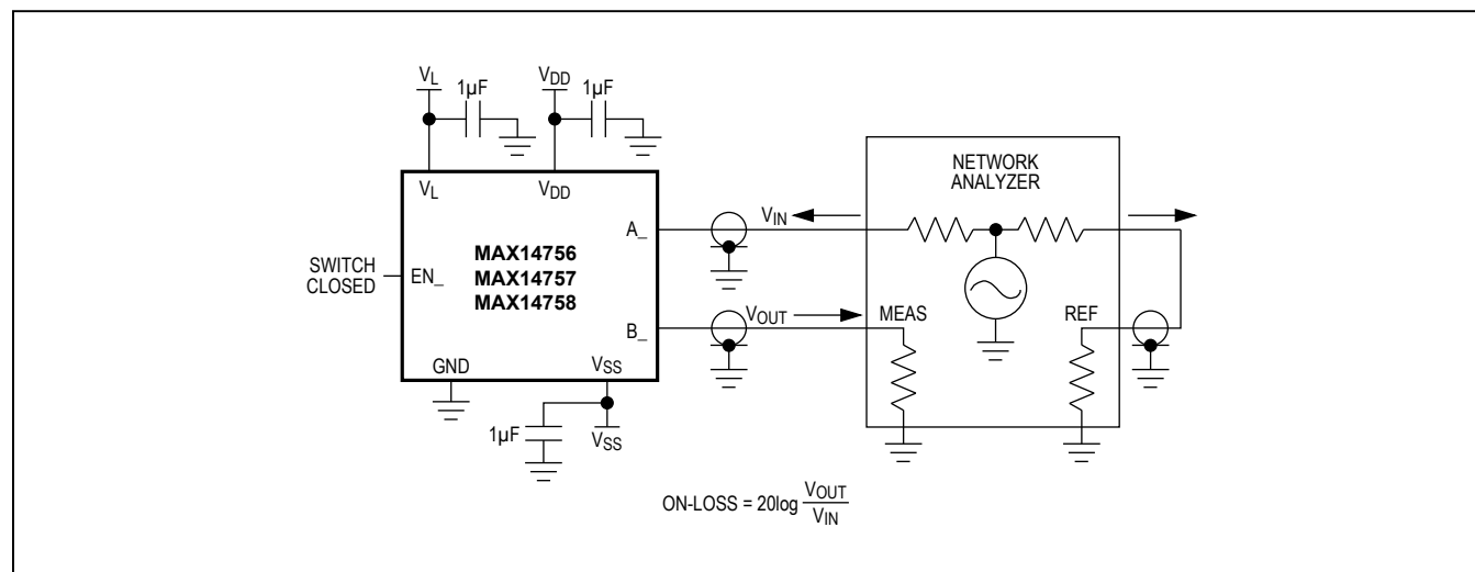
Figure 7. Frequency Response
