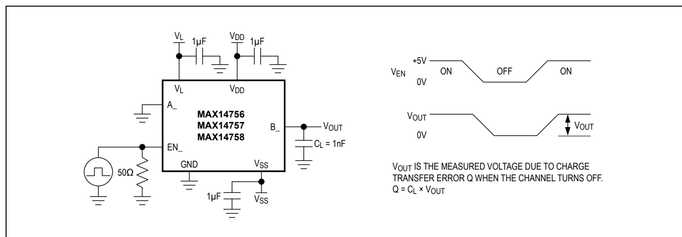
Figure 8. Charge Injection
