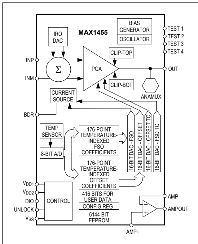
Figure 1. Functional Diagram
