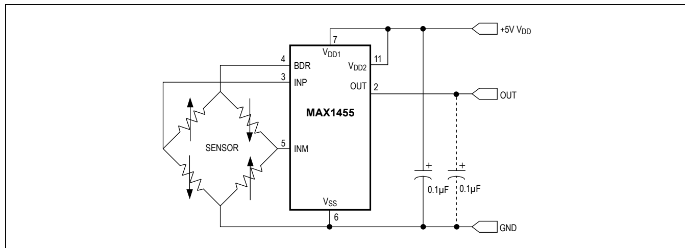
Figure 2. Basic Ratiometric Output Configuration
