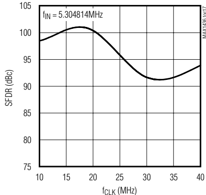
SPURIOUS-FREE DYNAMIC RANGE vs. SAMPLING RATE
