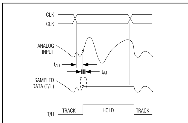
Figure 10. T/H Aperture Timing
