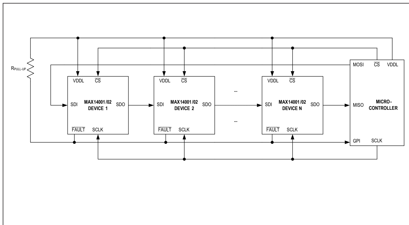
Figure 9. Daisy-Chain Connection
