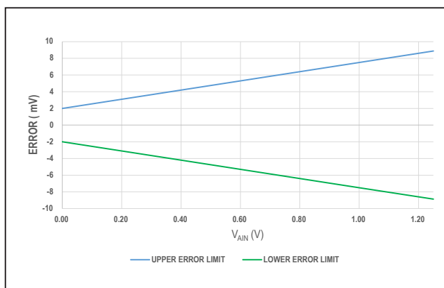
Figure 3. ADC Error Window (Excludes V_{\text{REF}} Error)
