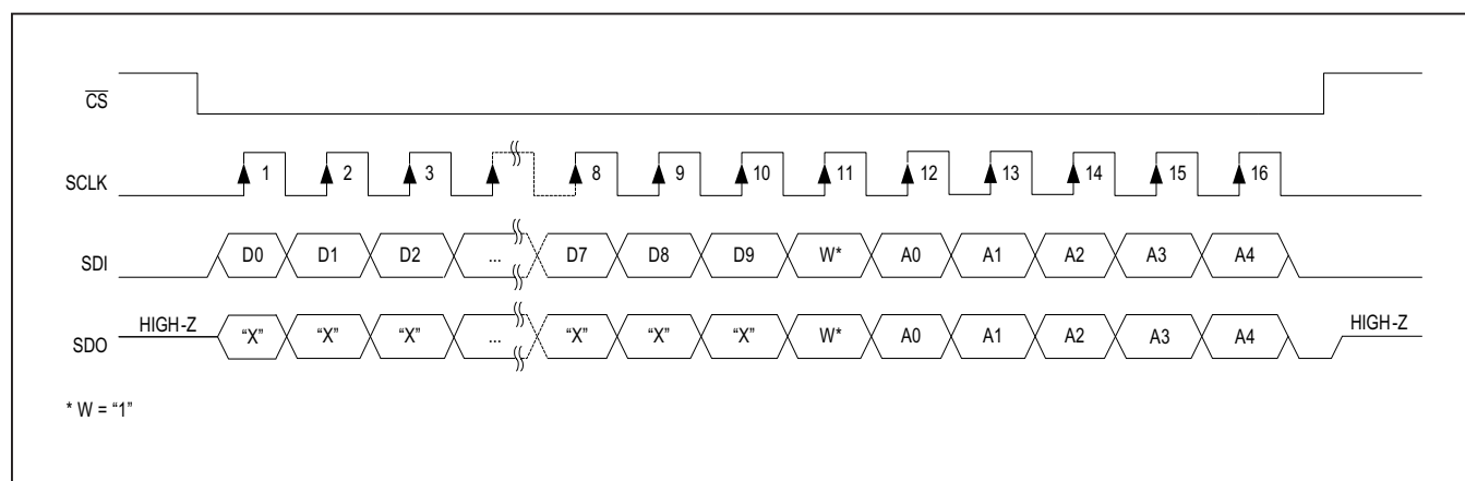
Figure 6. SPI Write
