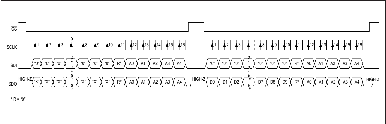
Figure 7. SPI Read
