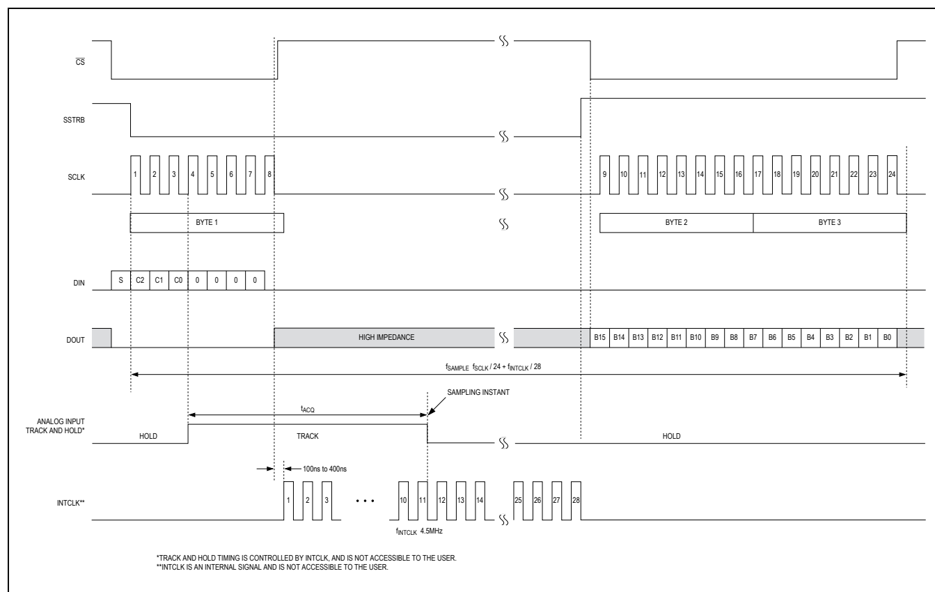
Figure 4. Internal Clock-Mode Conversion (Mode 2)
