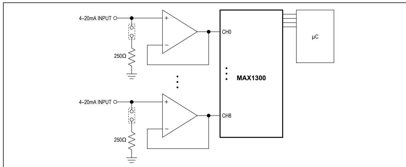
Figure 19. 4–20mA Application
