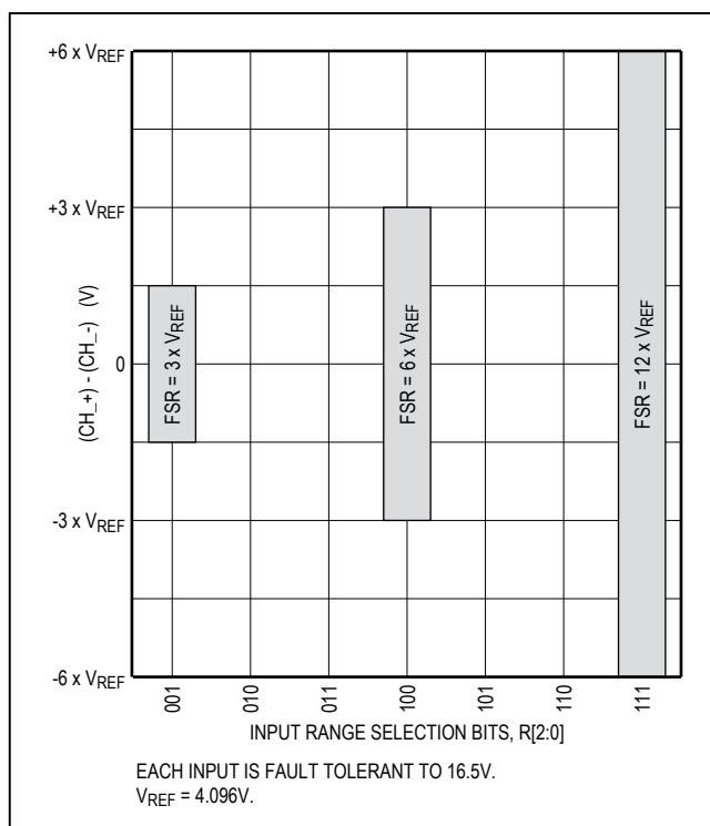
Figure 8. Differential Input Voltage Ranges
