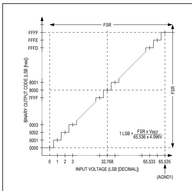
Figure 13. Ideal Unipolar Transfer Function, Single-Ended Input, -FSR to 0
