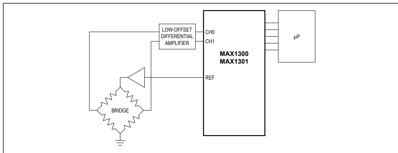
Figure 20. Bridge Application
