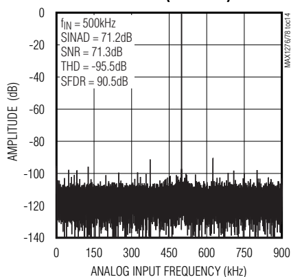
FFT PLOT (MAX1278)
