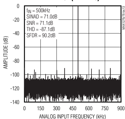
FFT PLOT (MAX1276)
