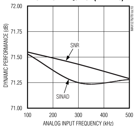
DYNAMIC PERFORMANCE vs. INPUT FREQUENCY (MAX1278)
