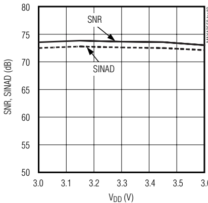
SNR, SINAD vs. ANALOG SUPPLY VOLTAGE ( f_{CLK} = 80MHz , f_{IN} = 70MHz )
