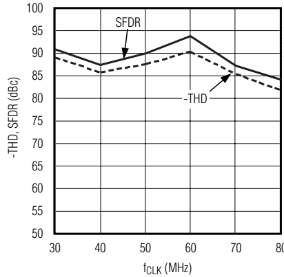
-THD, SFDR vs. CLOCK SPEED ( f_{IN} = 70MHz , A_{IN} = -1dBFS )
