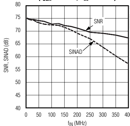
SNR, SINAD vs. ANALOG INPUT FREQUENCY (f_CLK = 80MHz, A_IN = -1dBFS)
