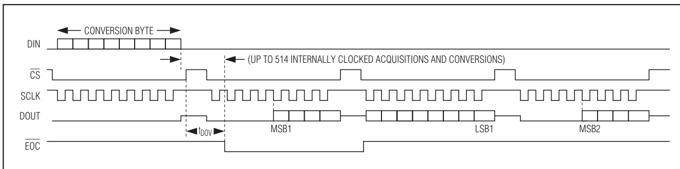
Figure 8. Clock Mode 10—The command byte to the conversion register begins the acquisition ( \overline{\text{CNVST}} is not required).
