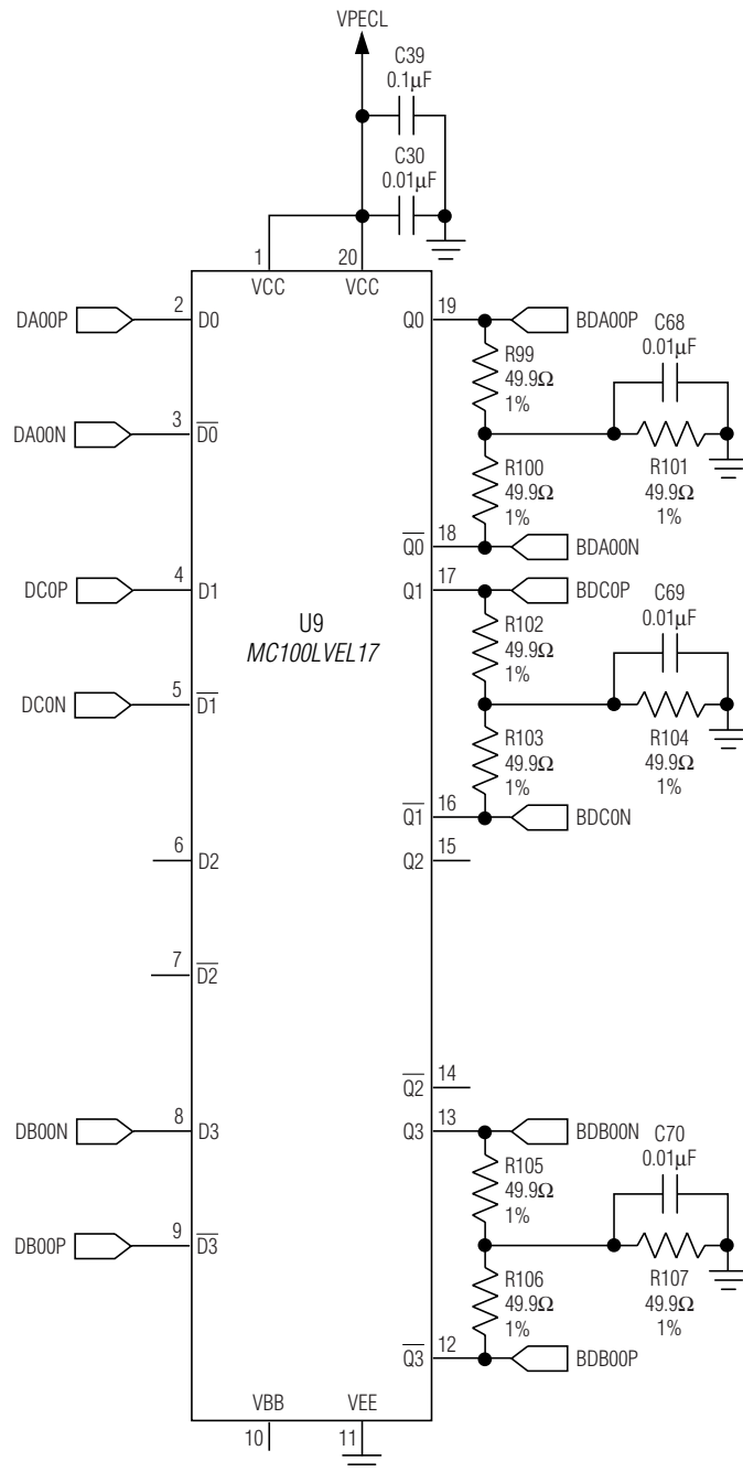
Figure 1i. MAX1217/MAX1218/MAX1219 EV Kit Schematic (Sheet 7 of 7)
