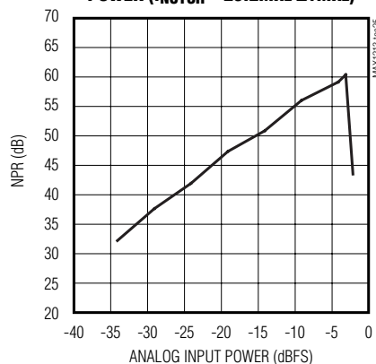
NOISE-POWER RATIO vs. ANALOG INPUT POWER ( f_{NOTCH} = 28.2MHz \pm 1MHz )
