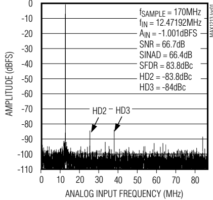
FFT PLOT (8192-POINT DATA RECORD)
