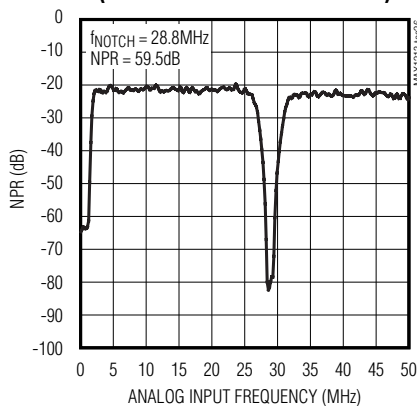
NOISE-POWER RATIO PLOT (WIDE NOISE BANDWIDTH: 50MHz)
