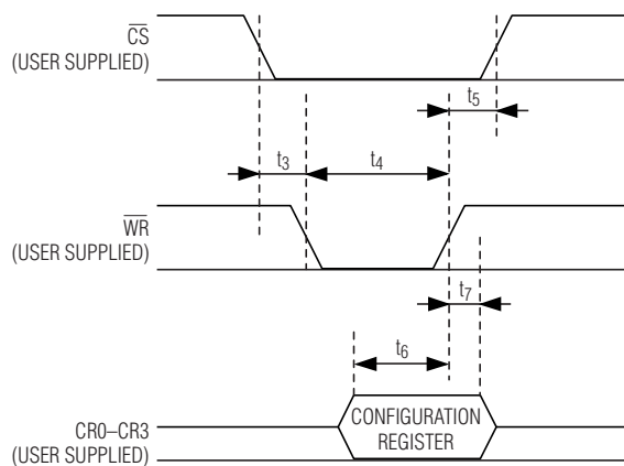
Figure 4. Programming Configuration-Register Timing Requirements
