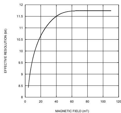
Effective Resolution (3σ)
