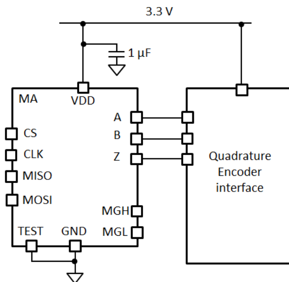
Figure 32: Typical Configuration Using ABZ Interface
