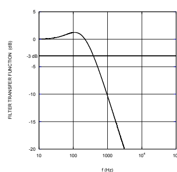
Filter Transfer Function
