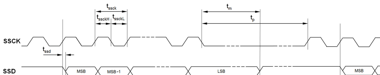
Figure 15: SSI Timing
