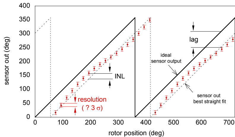
Figure A1: Resolution, INL, Lag
