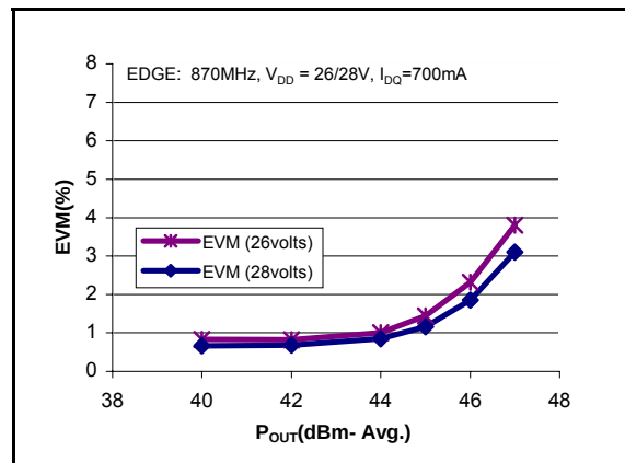
Graph 2. EDGE RMS EVM vs. Output Power
