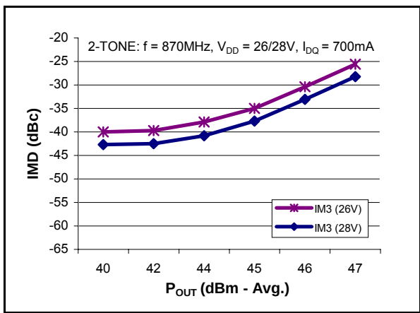
Graph 3. Two-Tone Intermodulation vs. Output Power
