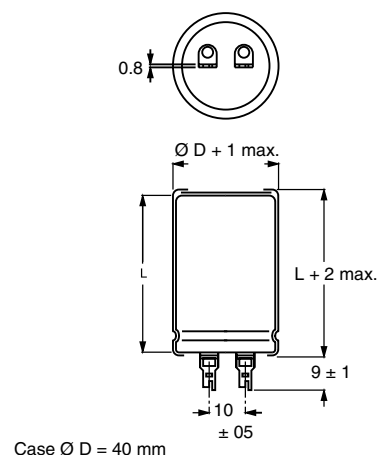
Fig. 10 Solder-lug version (SL): only available in 050 series
