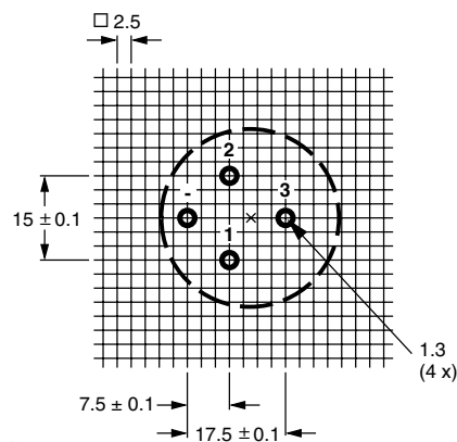
Case Ø D = 30 mm
