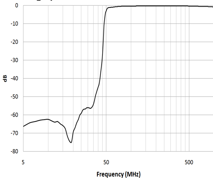
High pass filter insertion loss
