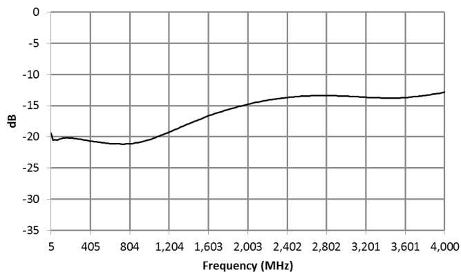
Coupling Return Loss (pin5)
