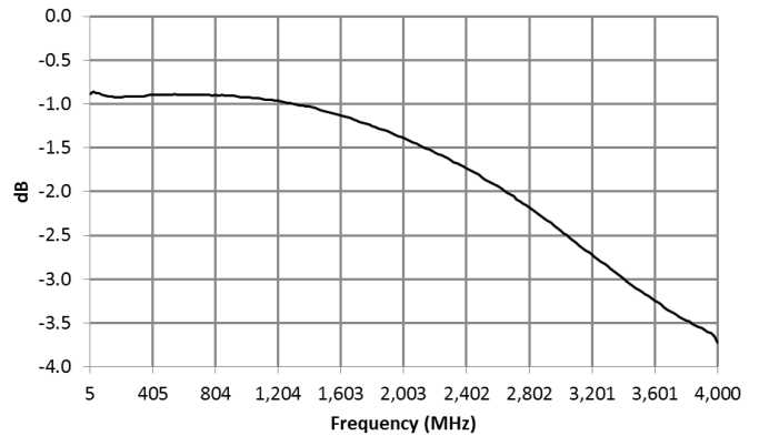
Main Line Loss (pin3-2)
