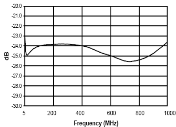
Coupled Port Return Loss
