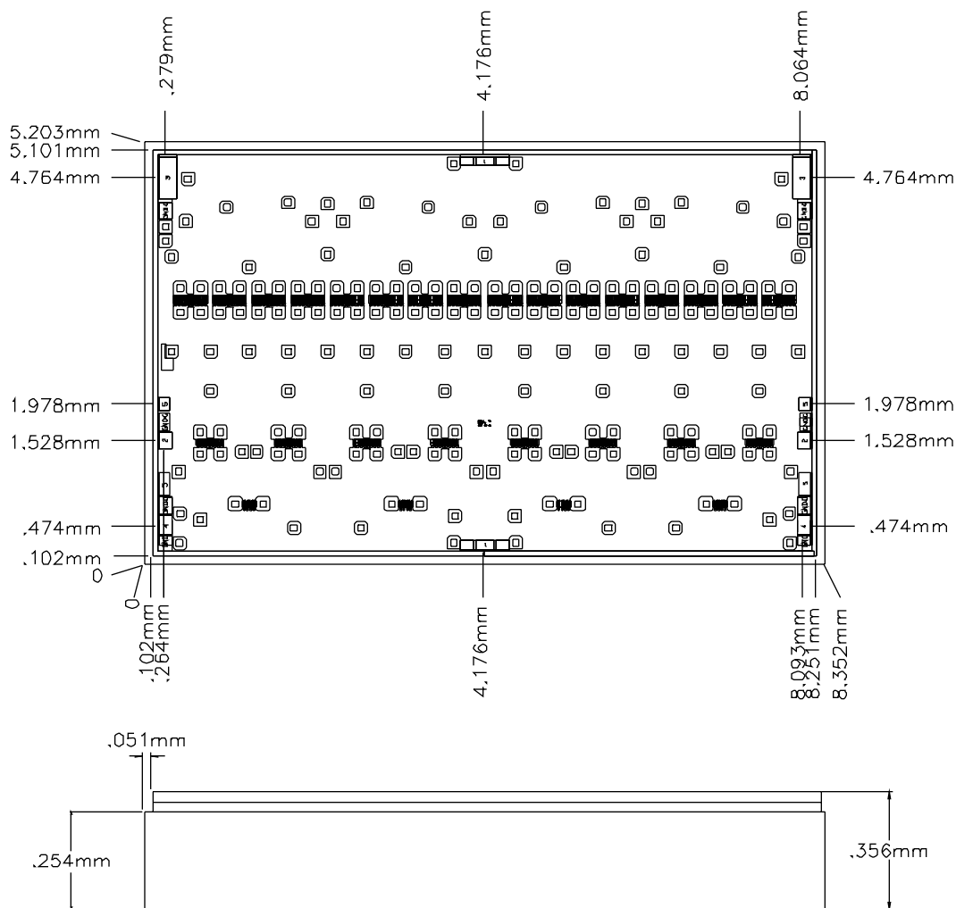
Figure 18. Die Layout
