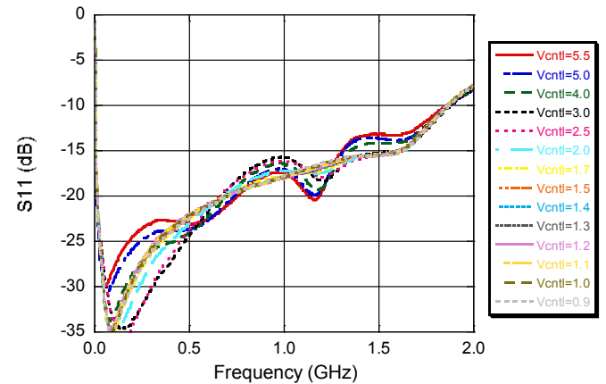
Input Return Loss vs. Frequency & VGA Control
