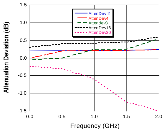
Attenuation Accuracy
