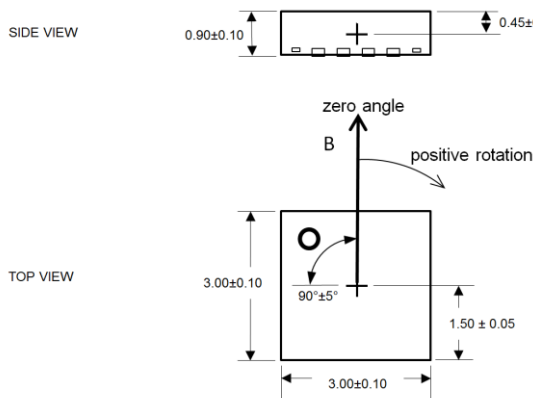
Figure 3: Zero Angle of Unprogrammed MA100
