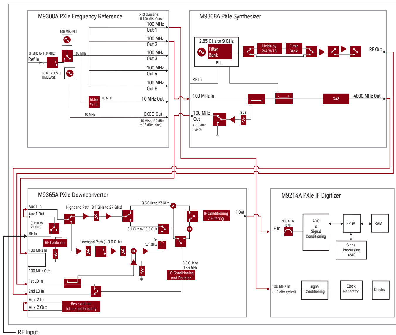
Figure 2. Standard M9393A PXIe vector signal analyzer (9 kHz to 27 GHz) block diagram with four modules consisting of the M9308A synthesizer, M9365A downconverter, M9214A digitizer and the optional M9300A frequency reference.
